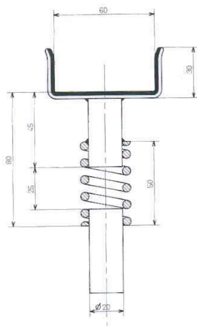
FIGURE 2: BLOC RESSORT
